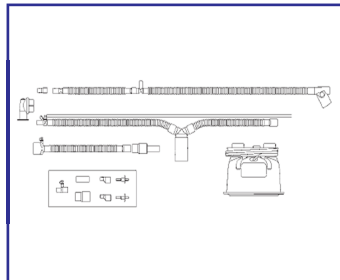
SLE 2000/ 5000 VENTİLATOR DEVRESİ
